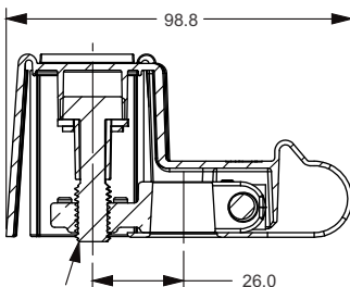
THREADLOCK ON THE BOLT THREADS RETENTION TORQUE DEGRADES WITH EACH DISASSEMBLY
