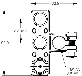
SHOWN WITHOUT COVER FOR REFERENCE
