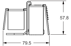
0FHZ0211Z Fuse & Stud Cover
