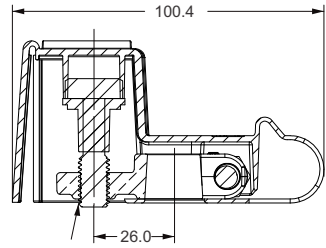
THREADLOCK ON THE BOLT THREADS RETENTION TORQUE DEGRADES WITH EACH DISASSEMBLY
