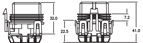
Cavity Plug
