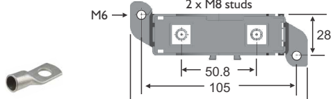
Mega M8 Tubular Terminals (see p188).
