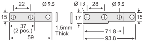
Midi Busbar Multiple Positions
